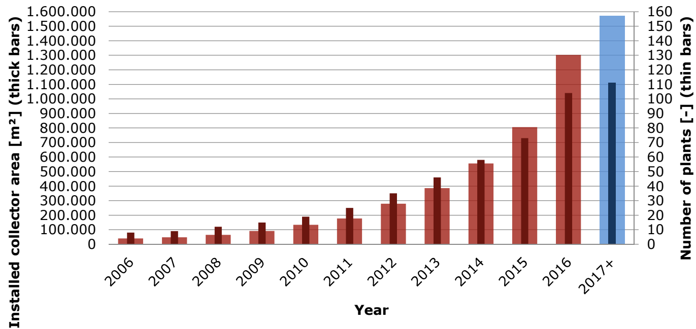
Solar District Heating in Denmark Sum of collector area and the number of operating and upcoming plants
